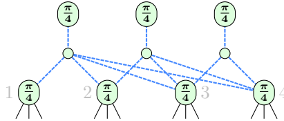
Figure 3.4: Diagram where the heuristic (3.16) underestimates the effective heuristic value
