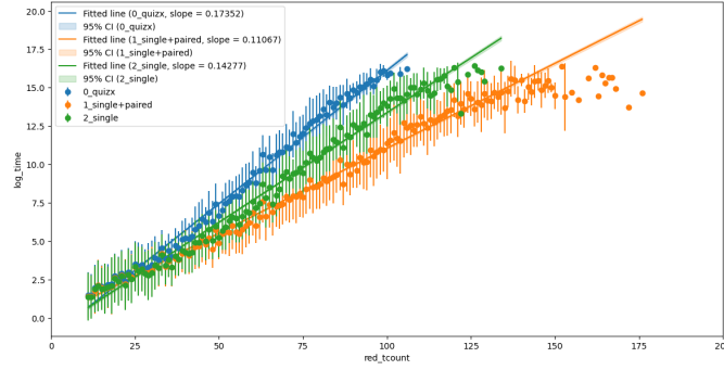
Figure 4.28: Mean log time (lower better) by T -count for Clifford+T circuits with CCZ
