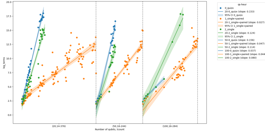
Figure 4.20: Mean log terms (lower better), separated by number of qubits, of modified hidden shift circuits
