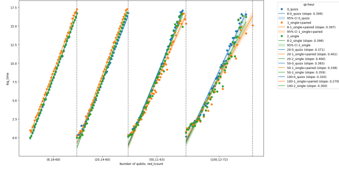
Figure 4.6: Mean log time (lower better) by T -counts, separated by number of qubits, for Clifford+T circuits
