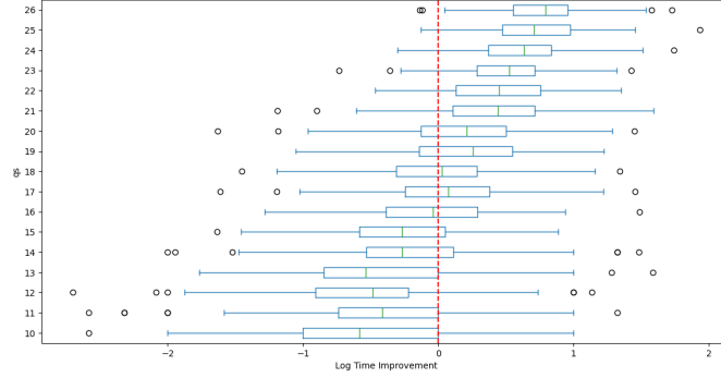
Figure 4.16: Improvement in log time ( single+paired vs. single ) for IQP circuits
