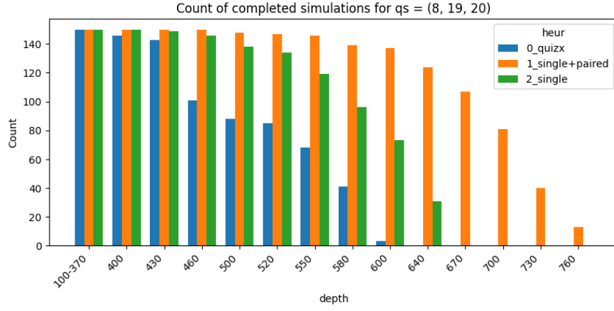
Figure 4.31: Number of completed simulations before timeout for q = 8, 19, 20 for Clifford+T circuits with CCZ
