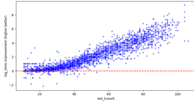
Figure 4.30: Improvement in log time (single+paired vs. quizx) for Clifford+T circuits with CCZ
