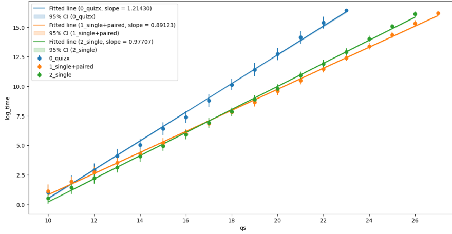
Figure 4.13: Mean log time (lower better) by number of qubits for IQP circuits
