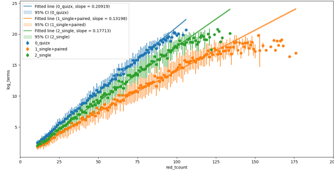
Figure 4.27: Mean log number of terms (lower better) by T -count for Clifford+T circuits with CCZ
