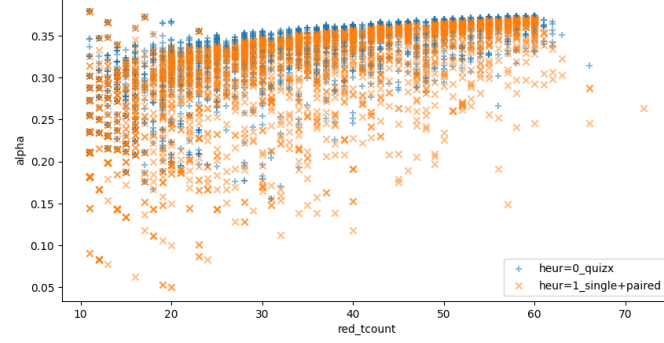
Figure 4.2: \alpha values (lower better) for Clifford+T circuits
