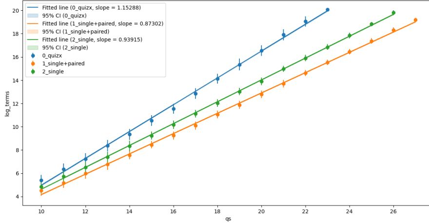
Figure 4.14: Mean log terms (lower better) by number of qubits for IQP circuits
