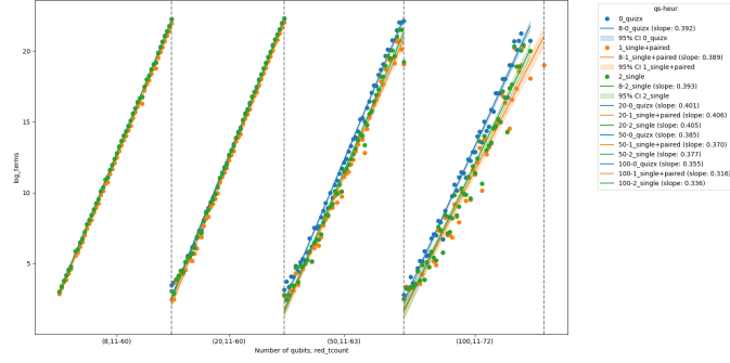
Figure 4.5: Mean log number of terms (lower better) by T -counts, separated by number of qubits, for Clifford+T circuits
