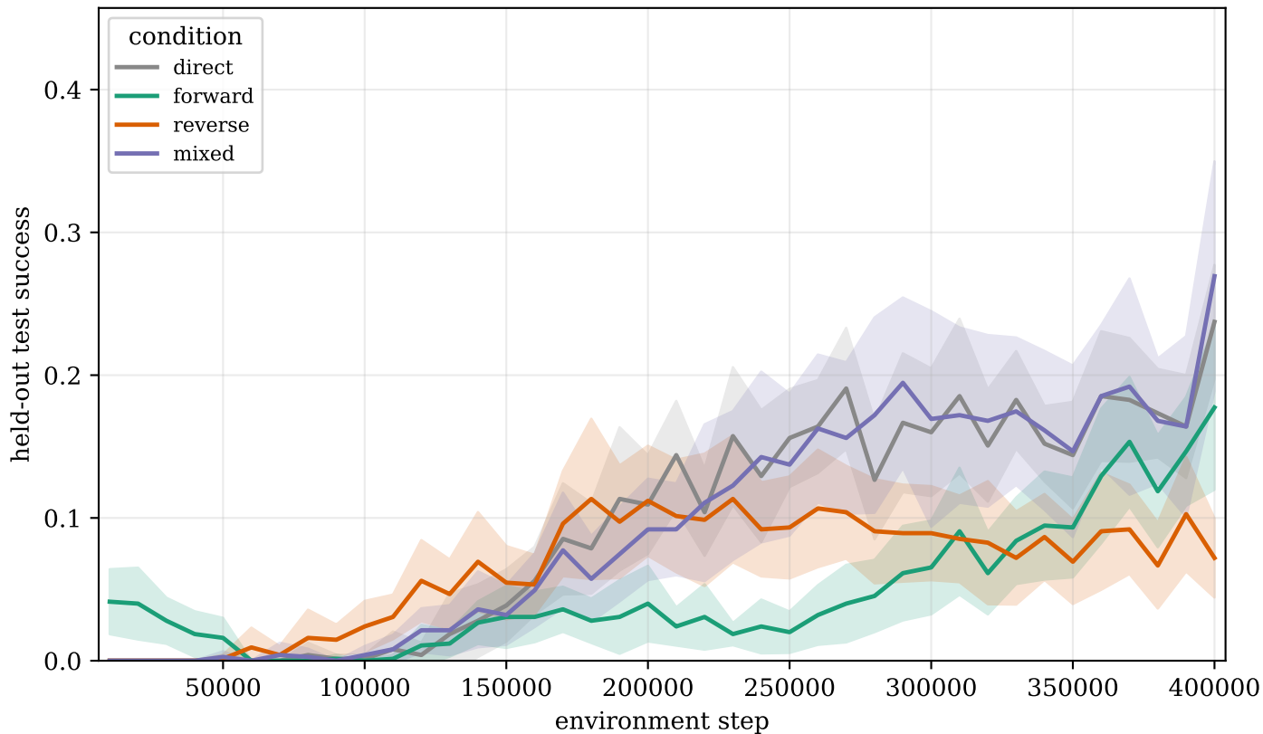
Curriculum strategy on 6x6/1L (pooled over algorithms, n=15, 95% CI)
