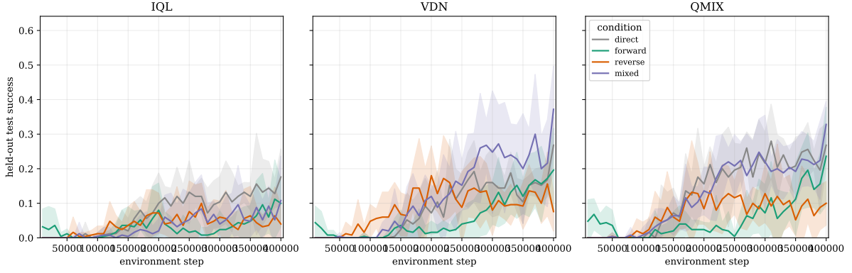
Figure 21: The same held-out test learning curves as Figure 20, shown per algorithm (IQL, VDN, QMIX) rather than pooled. Interim: n = 5 of a planned 20 seeds.
