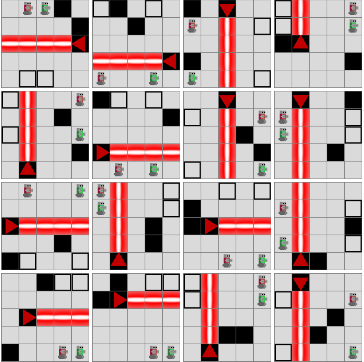
Figure 35: 16 Constructive Cooperative 5x5 (2 agents, 1 laser) levels.
