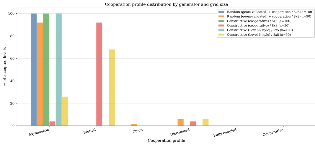
Figure 15: Distribution of cooperation profiles among accepted cooperative levels, grouped by generator and grid size. Each bar shows the fraction of accepted levels assigned to a given profile family.
