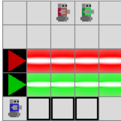
Figure 4: mutual: two stacked beams of distinct colours. Each agent is immune to its own beam but must wait for the other to truncate the foreign beam before crossing. Edges: \{(0, 1), (1, 0)\} .
