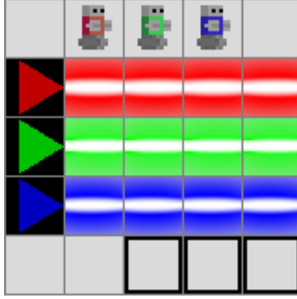
Figure 7: fully_coupled : three agents and three beams stacked, so every agent must shield, and be shielded by, both others to reach the bottom row of exits. The complete dependency graph has all six edges between distinct agents. Edges: \{(0, 1), (0, 2), (1, 0), (1, 2), (2, 0), (2, 1)\} .
