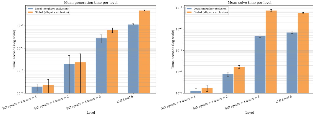
Figure 11: SAT solver time (seconds) for the global and local uniqueness formulations across the four benchmark levels.
