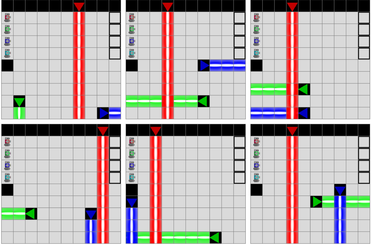
Figure 21: Six representative training levels from curriculum stage 3 ( 10 \times 10 , 4 agents, 3 lasers, T_{\max} = 18 , generator cooperative).
