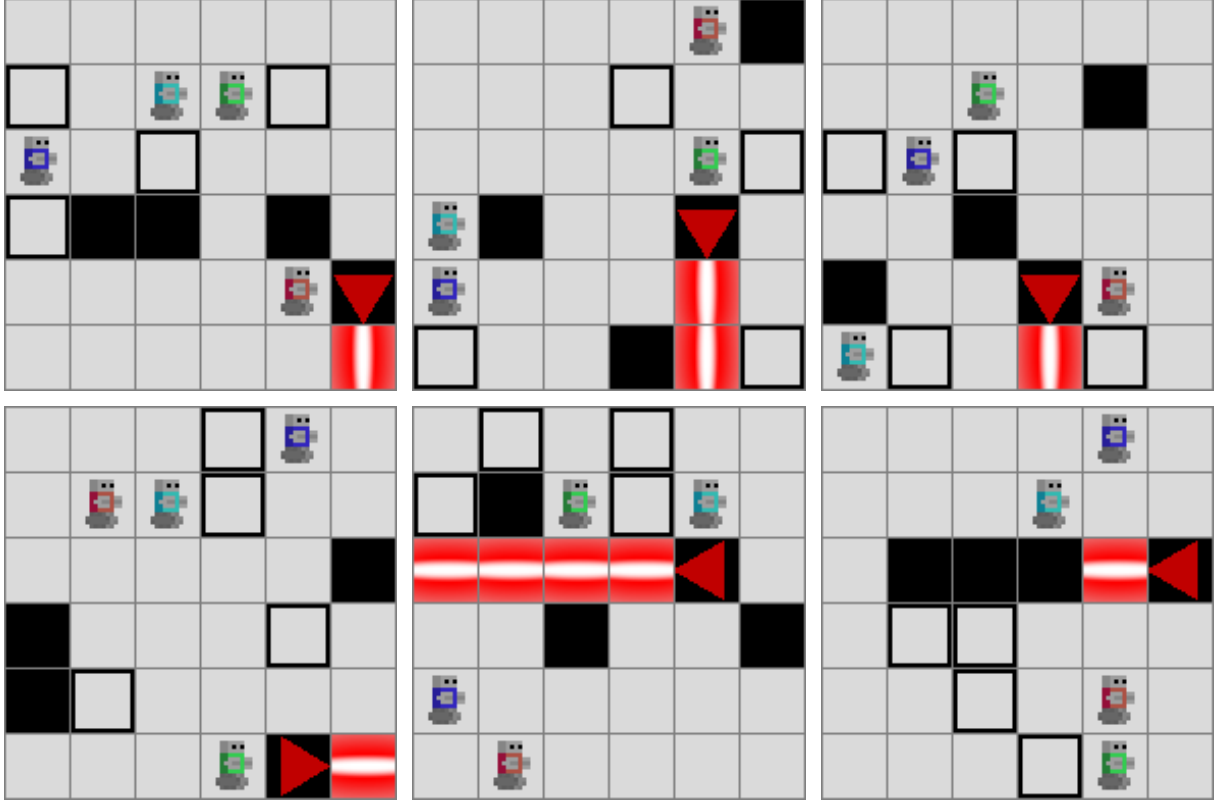
Figure 19: Six representative training levels from curriculum stage 1 ( 6 \times 6 , 4 agents, 1 laser, T_{\max} = 12 , generator random).
