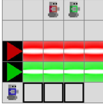
Figure 5: mutual : two stacked beams of distinct colours. Each agent is immune to its own beam but must wait for the other to truncate the foreign beam before crossing. Edges: \{(0, 1), (1, 0)\} .
