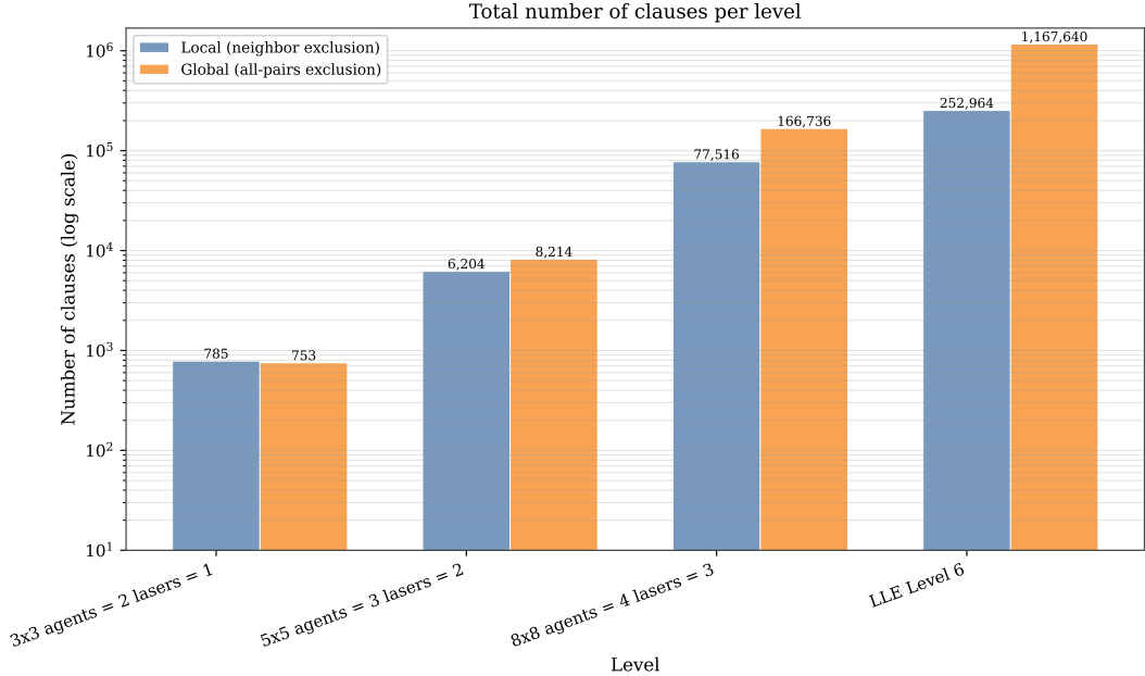
Figure 11: Number of clauses generated by the global and local uniqueness formulations across the four benchmark levels. The vertical axis is logarithmic because clause counts span more than three orders of magnitude.
