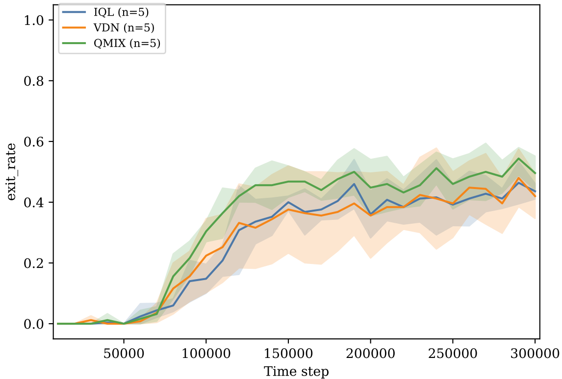
Success rate (train set)
