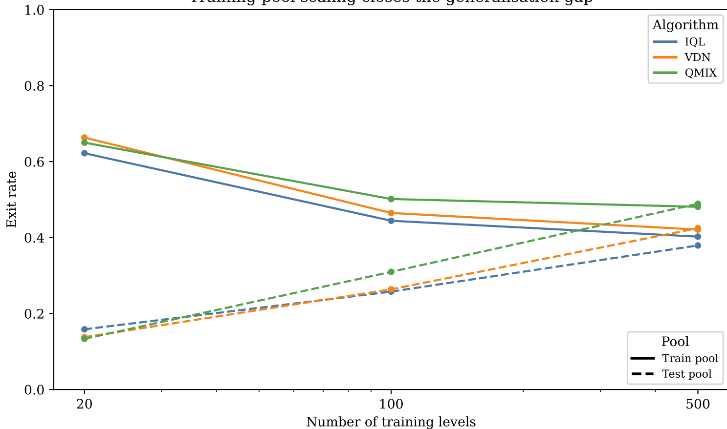
Training-pool scaling closes the generalisation gap
