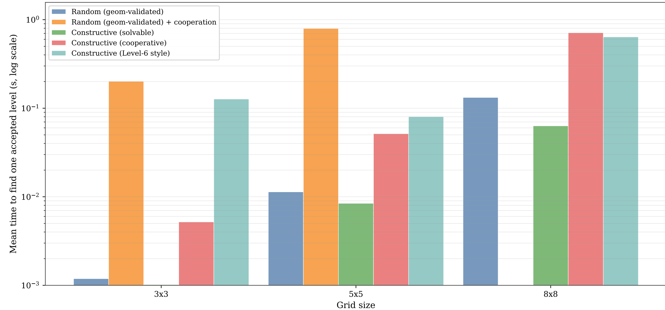
Mean time per accepted level by generator and grid size
