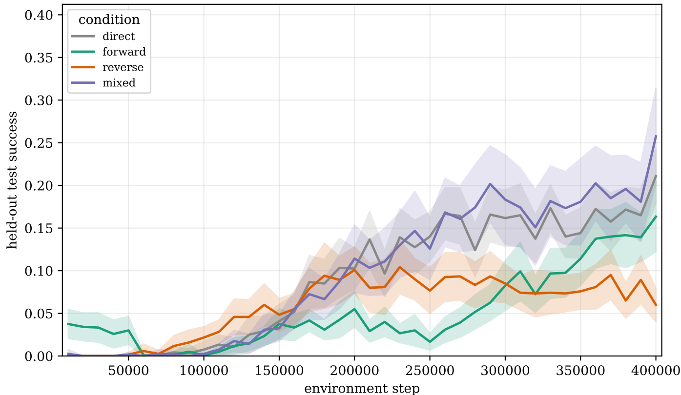
Curriculum strategy on 6x6/1L (pooled over algorithms, n=24, 95% CI)
