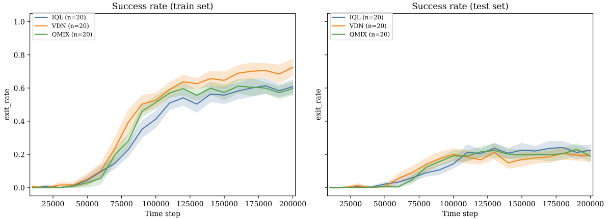
Figure 10: Mean success rate (greedy exit rate) on the training and held-out test pools as a function of environment steps, for IQL, VDN, and QMIX. Shaded bands are 95 % confidence intervals over the twenty training seeds, clipped to the per-step minimum and maximum.
