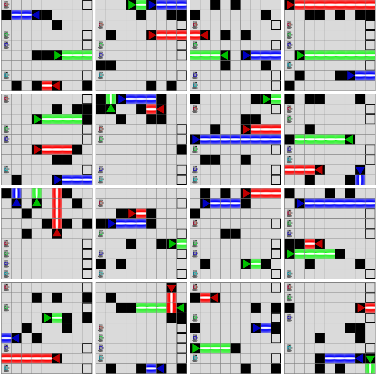
Figure 45: 16 Constructive Solvable 9 \times 9 (4 agents, 3 lasers) levels.
