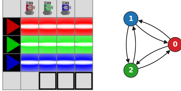
Figure 8: fully_coupled: three agents and three beams stacked, so every agent must shield, and be shielded by, both others to reach the bottom row of exits. The complete dependency graph has all six edges between distinct agents. Edges: \{(0, 1), (0, 2), (1, 0), (1, 2), (2, 0), (2, 1)\} .
