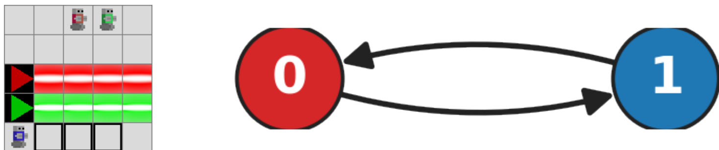
Figure 5: mutual: two stacked beams of distinct colours. Each agent is immune to its own beam but must wait for the other to truncate the foreign beam before crossing. Edges: \{(0, 1), (1, 0)\} .
