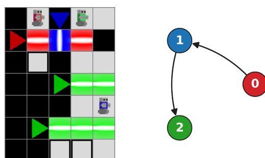
Figure 6: chain: three agents and two beams. Walls confine each agent to a separate region so helping flows in one direction only — red helps blue across the red beam, blue helps the third agent across the blue beam. Edges: \{(0, 1), (1, 2)\} .
