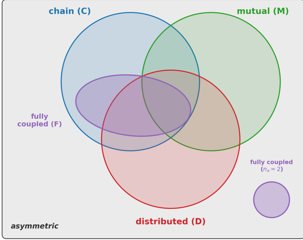
Figure 9: Cooperation patterns on the dependency graph G_L (for n_a \geq 3 ), as an Euler diagram of substructure containment. Chain (C), distributed (D), and mutual (M) are three overlapping circles. Fully coupled (F) lies inside chain and covers C \cap D \cap M , C \cap D , and the chain-only region, but not the chain-and-mutual-without-distributed lens, which is empty because F \cap M \subseteq D . The two-agent fully-coupled case (the reciprocal pair, which contains no chain) is drawn as a separate circle. The residual area outside every circle is asymmetric.
