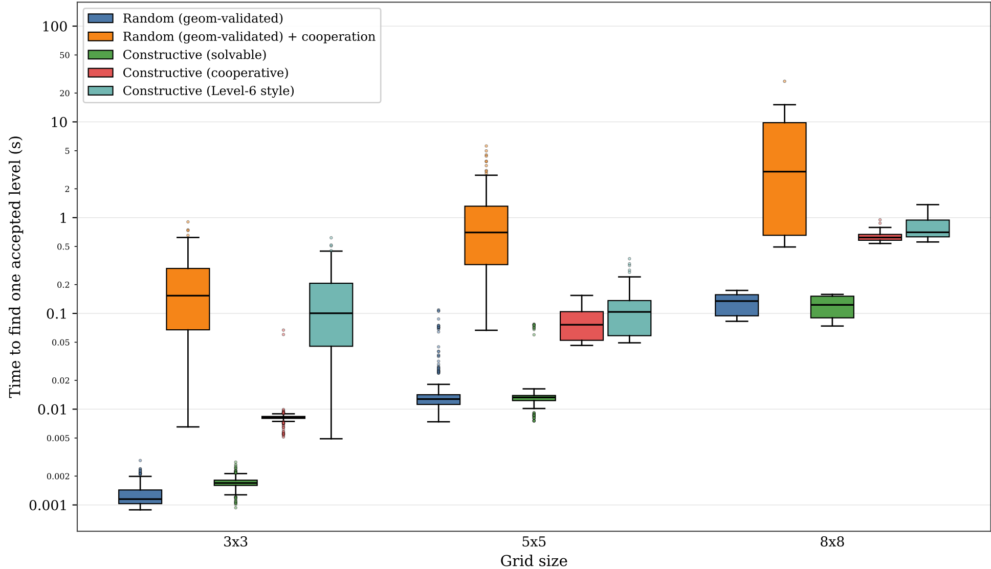
Time to find one accepted level by generator and grid size
