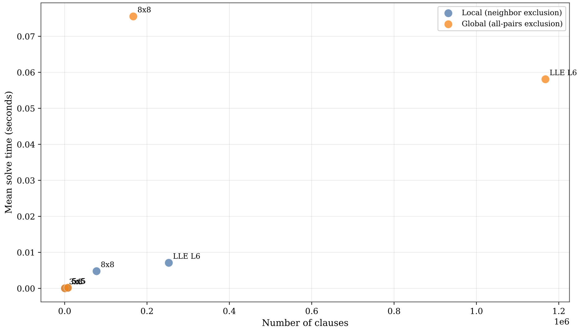
Clauses vs solve time
