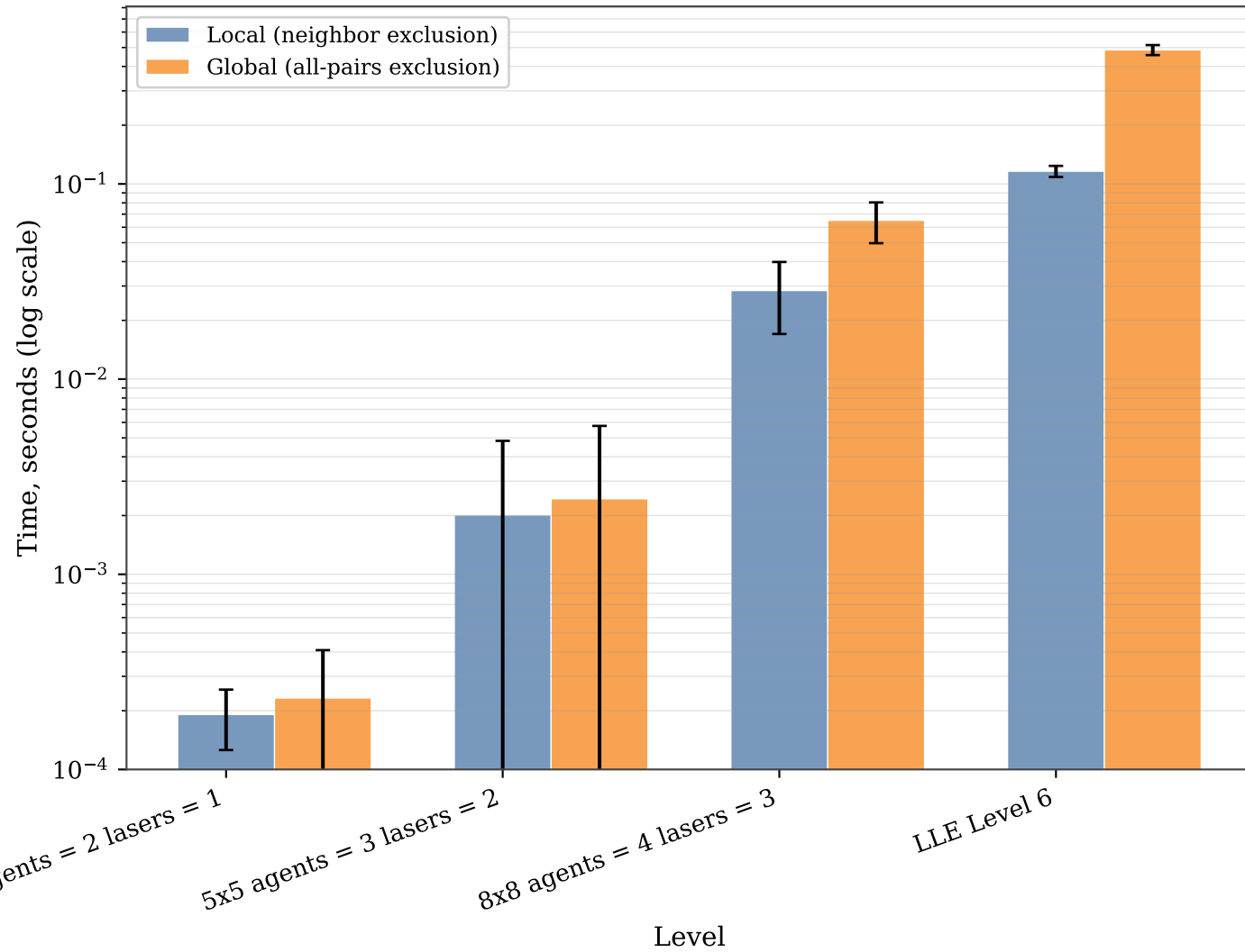
Mean generation time per level
