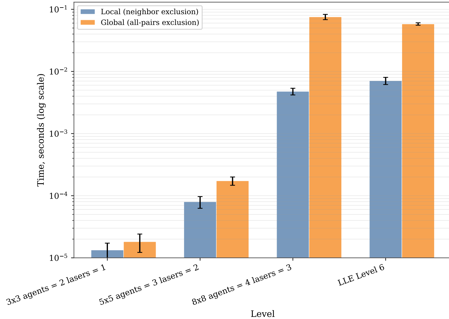
Mean solve time per level
