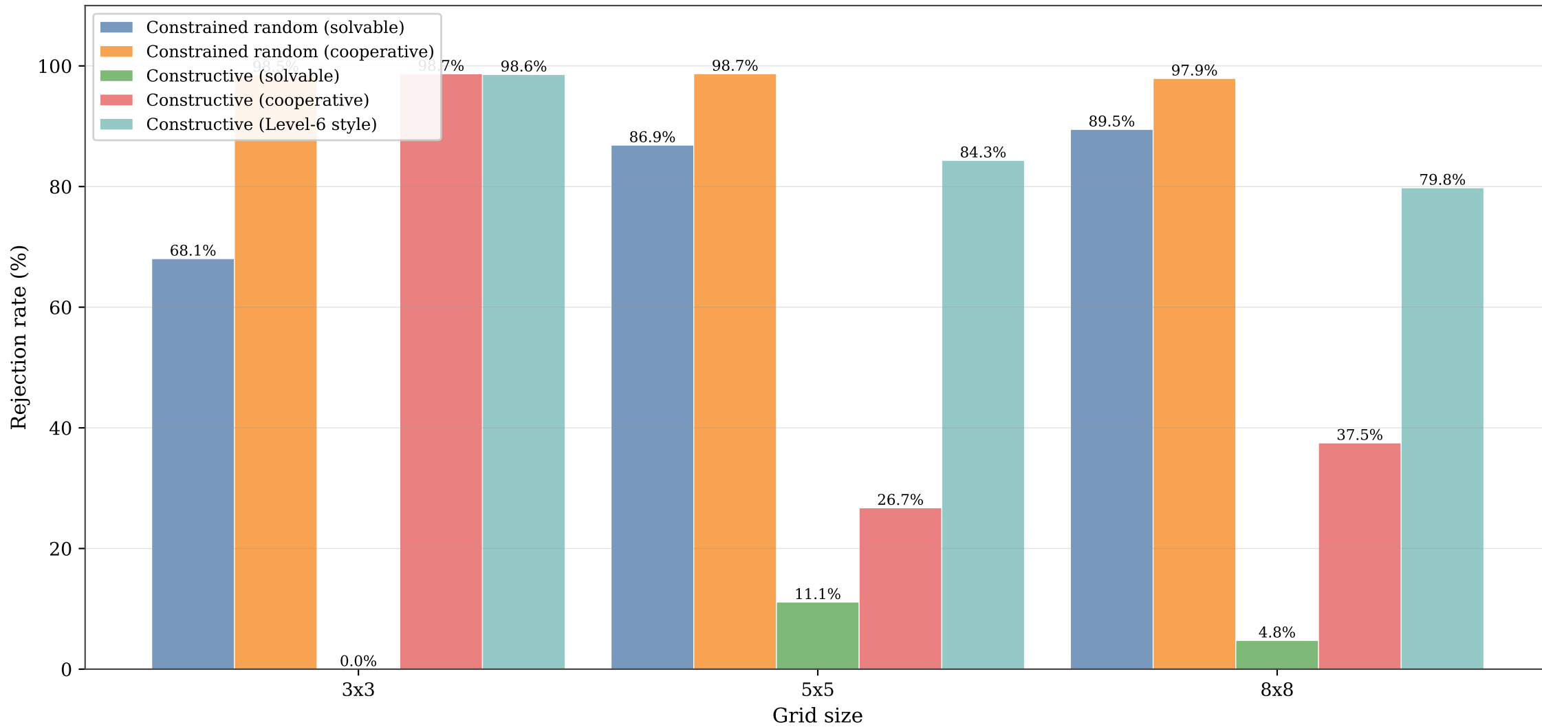
Rejection rate by generator and grid size
