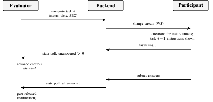
Fig. 2. Two-way gating during a moderated session. The participant follows the evaluator over a realtime channel; the evaluator’s gate is refreshed by short-interval polling of the same persisted state, so either client can reload mid-session and rejoin consistently.
