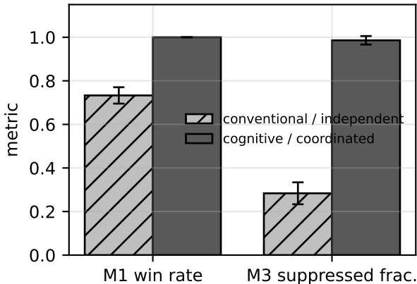
Cognitive policy vs. baseline (5 seeds)
