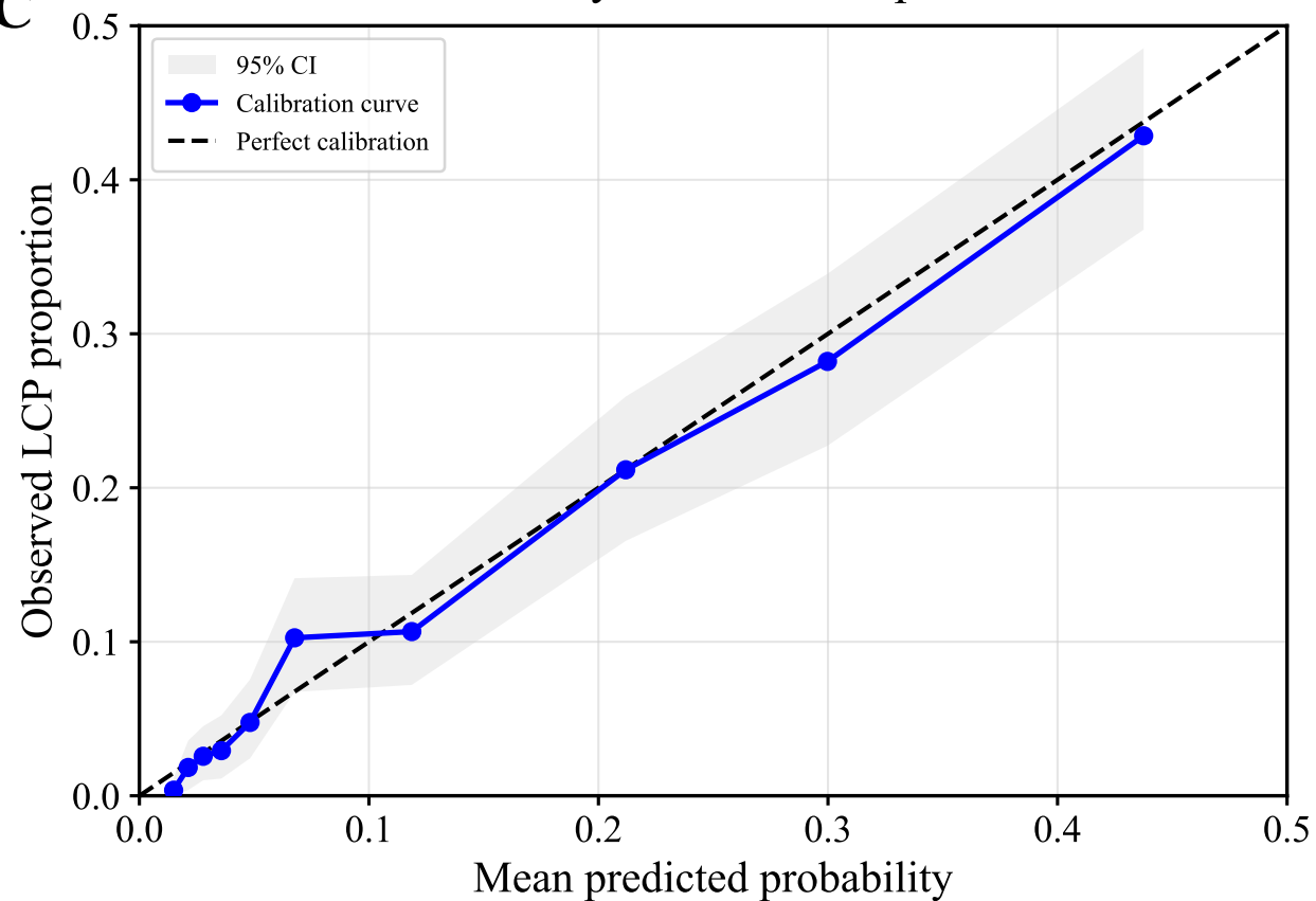
Calibration curve of survey-defined LCP prediction in CHARLS
