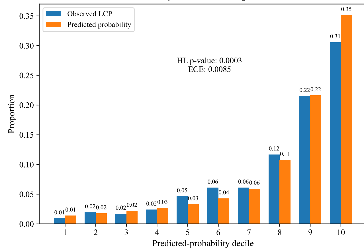
Calibration curve of survey-defined LCP prediction in CFPS
