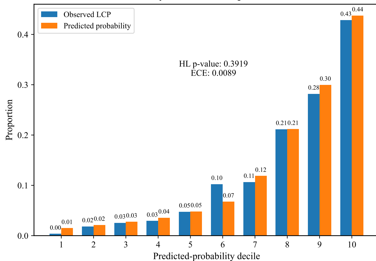
Calibration curve of survey-defined LCP prediction in CHARLS
