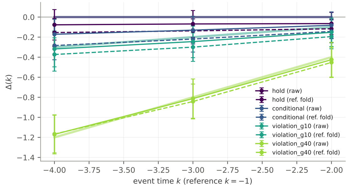
(b) Estimated vs true \Delta(k)
