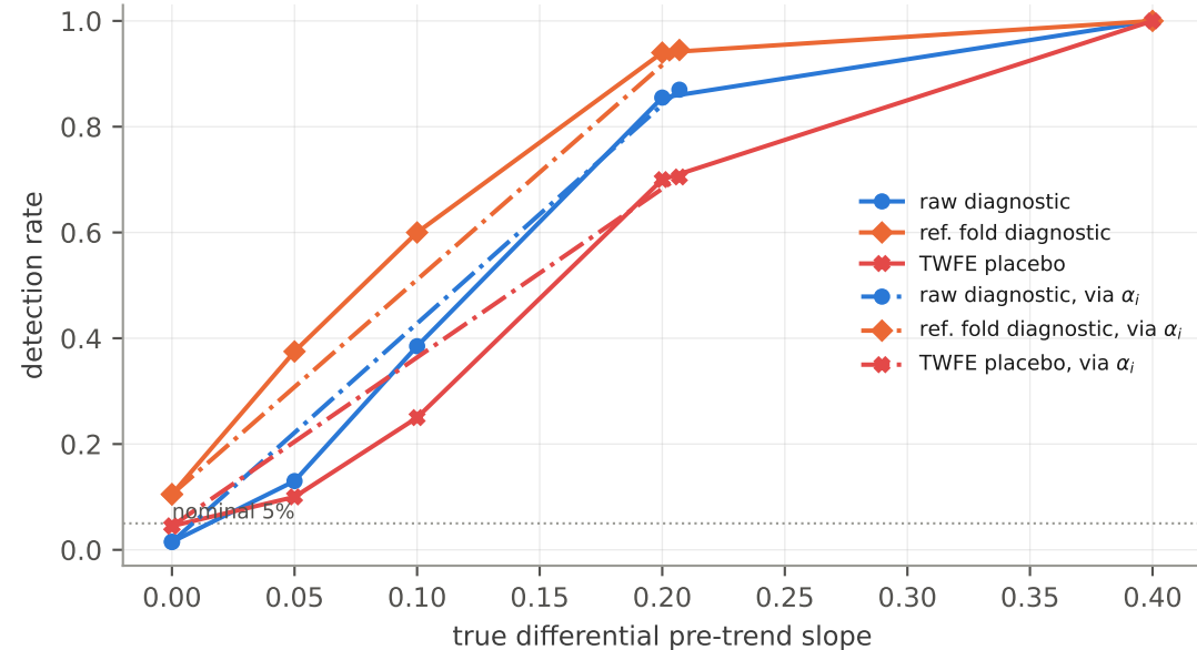
(a) Size at 0, power beyond
