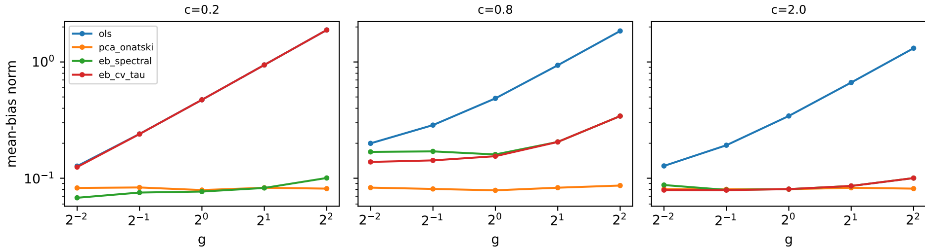
Crossover strip: bias vs confounding strength
