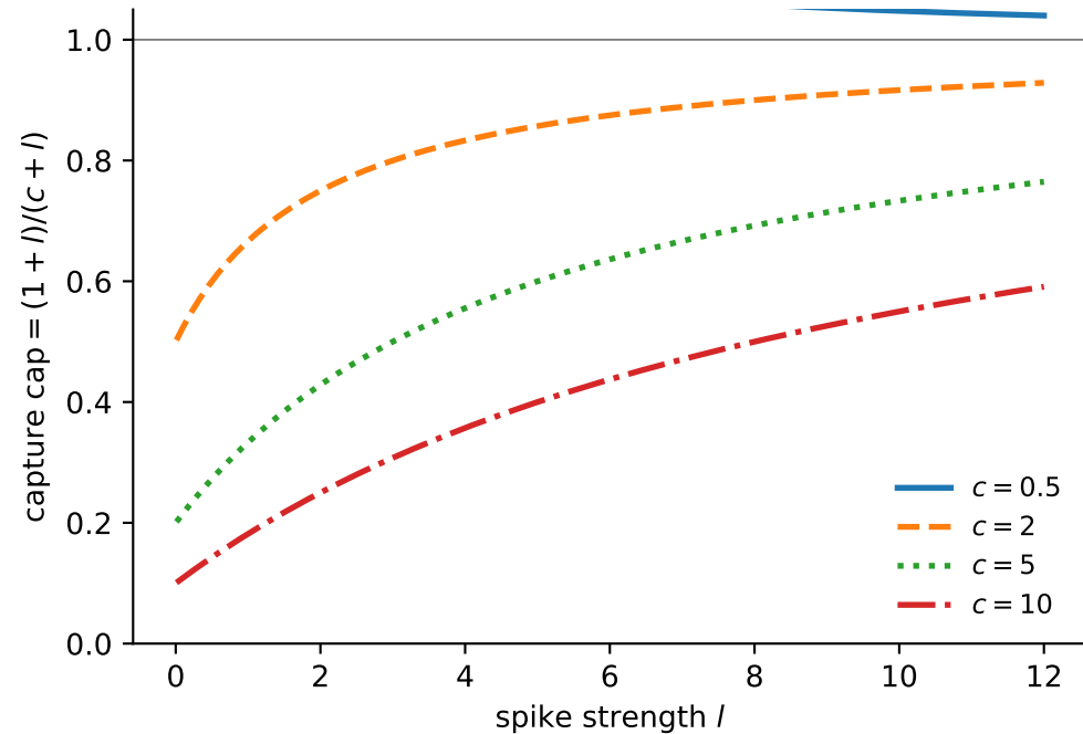
(a) The capture law
