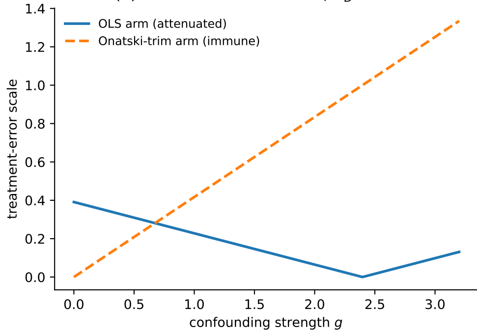
(b) Trimmed- \tau law at c = 2 , \Lambda_D = 1.558
