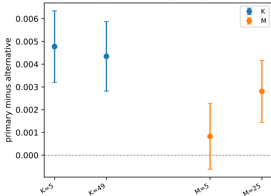
IC1: paired improvement vs primary (LAW-A-K)
