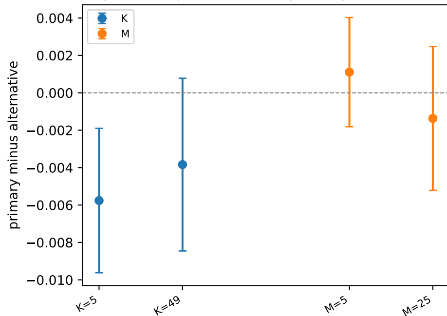
IC3: paired improvement vs primary (LAW-A-K)
