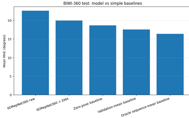
Figure 3: Simple baseline comparison. Constant predictors are competitive because roll and pitch are relatively centred in BIWI-360, while zero-shot predictions contain large outliers.
