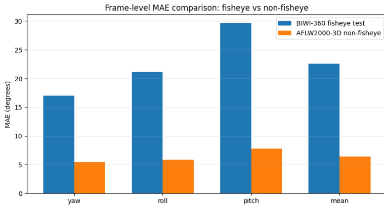
Figure 1: Sanity-check comparison between BIWI-360 and AFLW2000-3D. The same model performs much better on non-fisheye images, supporting the domain-shift interpretation.
