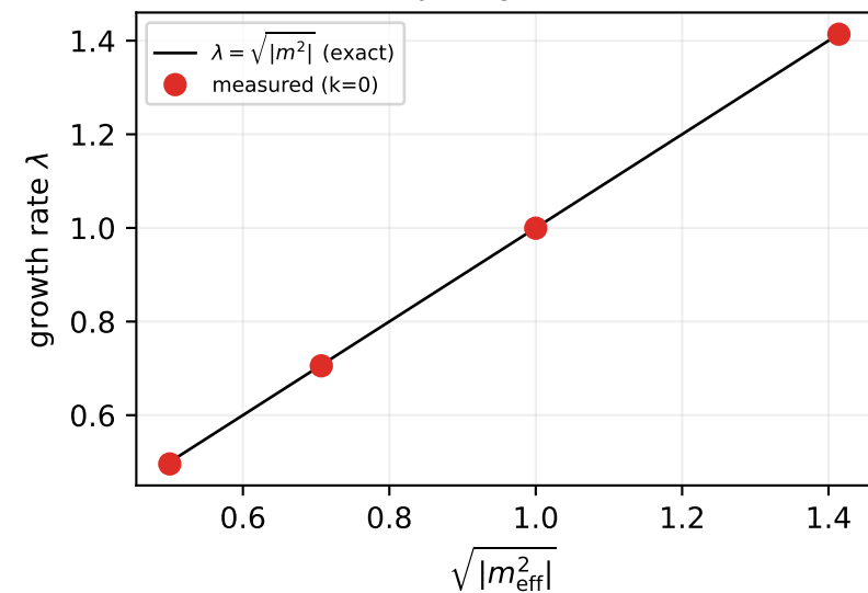
Tachyonic growth rate
