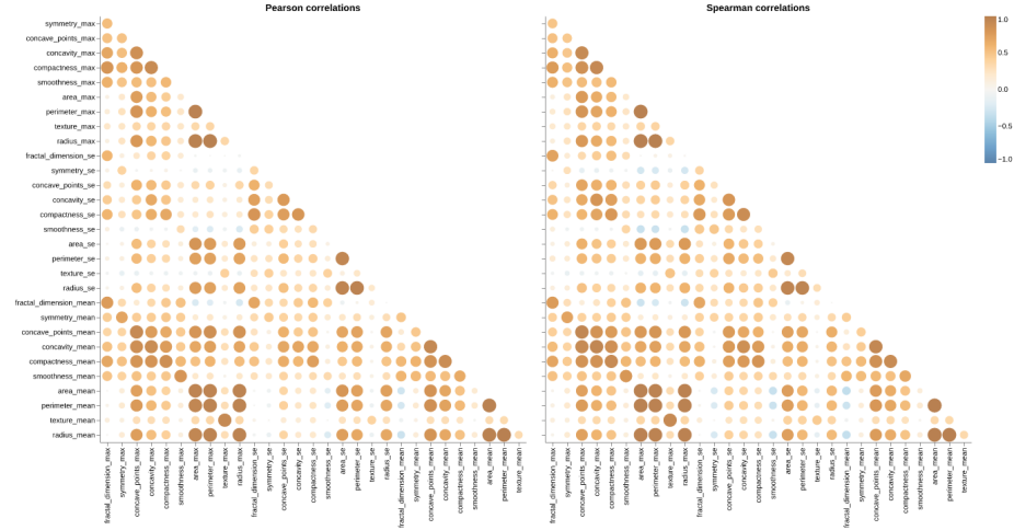
Figure 1: Multicollinearity
