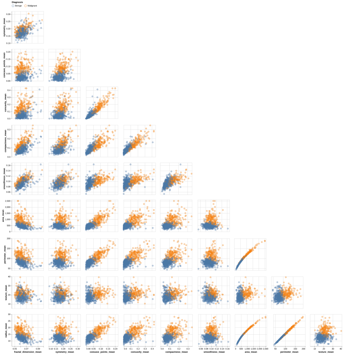
Figure 6: Pairwise Separability
