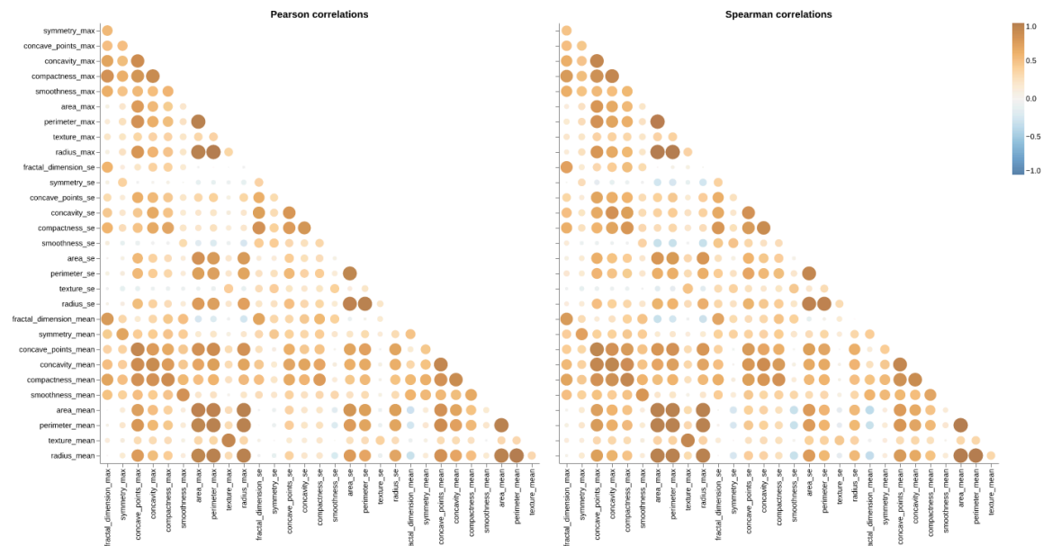
Figure 5: Multicollinearity
