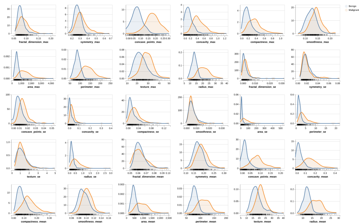
Figure 7: Distribution Analysis
