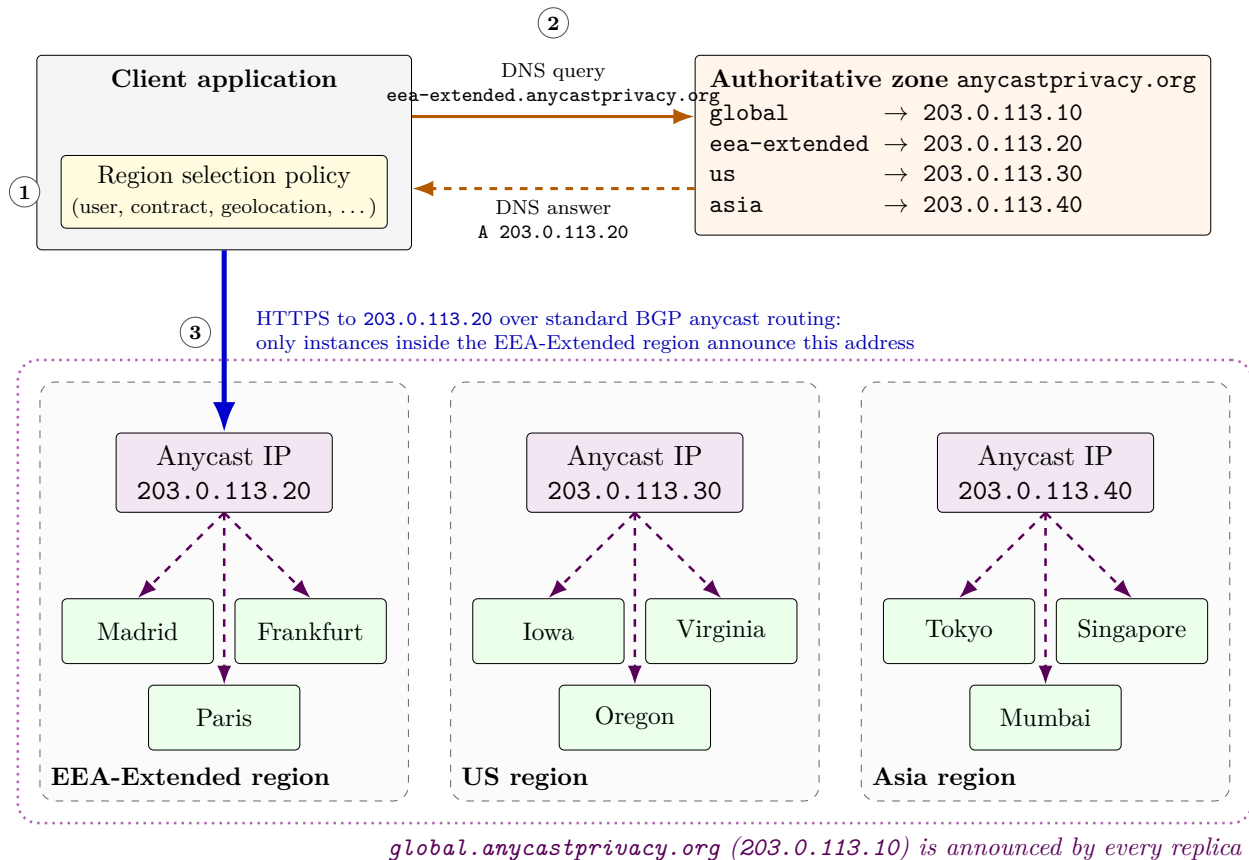
Figure 5.1: RCA-DNS architecture. (1) The client application selects a region according to its policy; (2) it resolves the name associated with that region, which always returns the same regional anycast address; (3) traffic is delivered by standard BGP anycast routing to one of the replicas that serve that address, all of which are located inside the selected region.
