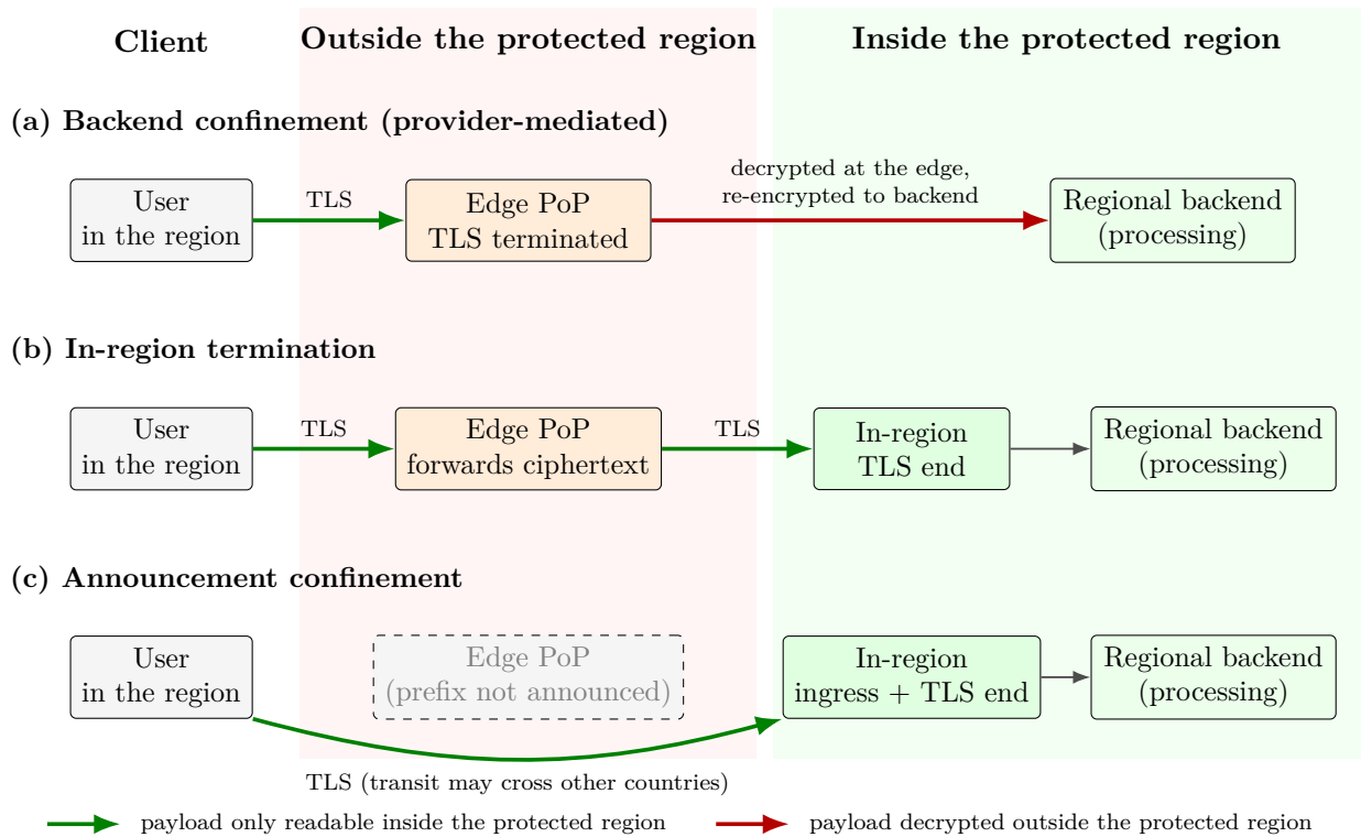
Figure 5.4: Levels at which an RCA-DNS deployment can enforce geographic confinement, for a user located in the protected region whose traffic would enter the provider’s network outside it.
