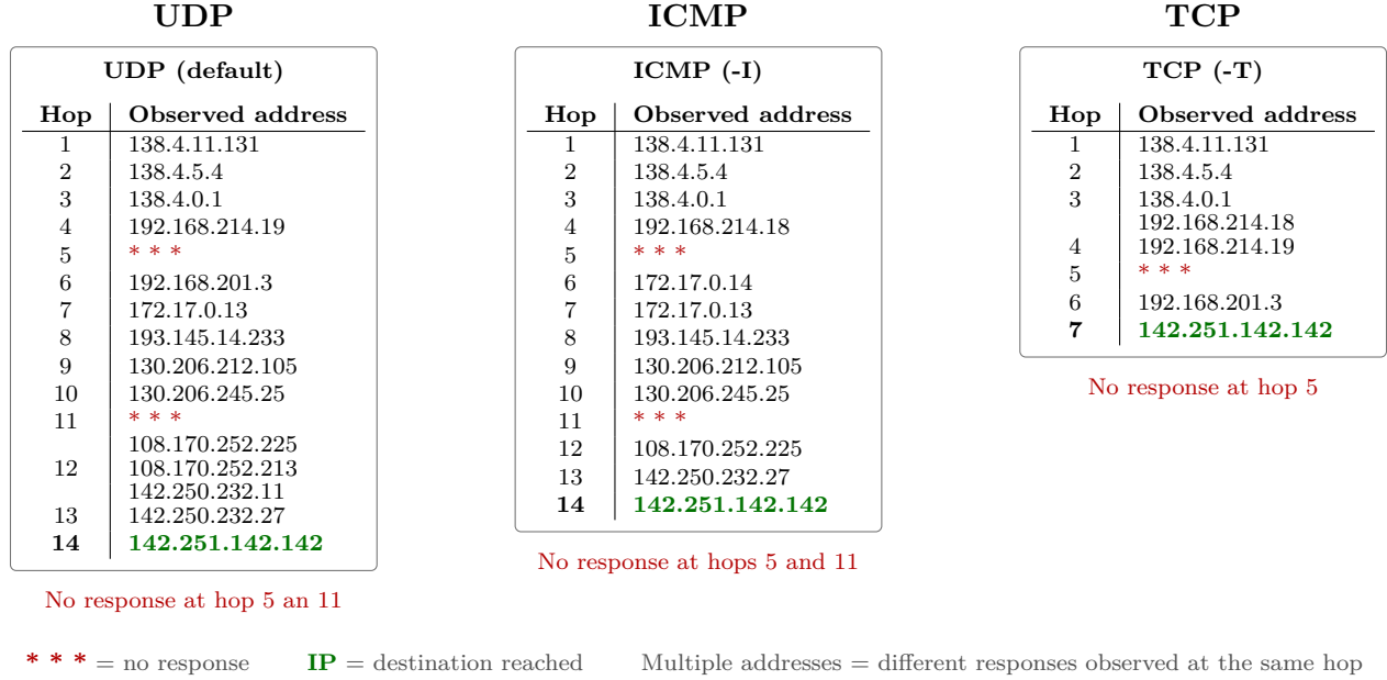
Figure 3.2: Comparison of traceroute measurements using UDP, ICMP, and TCP probes towards the same destination. The measurements exhibit different observable paths depending on the selected protocol.
