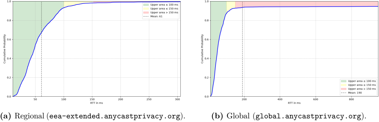
Figure 5.7: Cumulative distribution of the RTT observed by probes located in EEA-Extended countries when accessing the service through the regional deployment and through the conventional global deployment.
