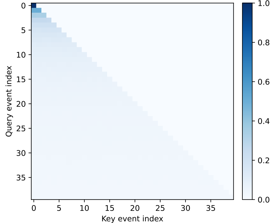
RoTHP
