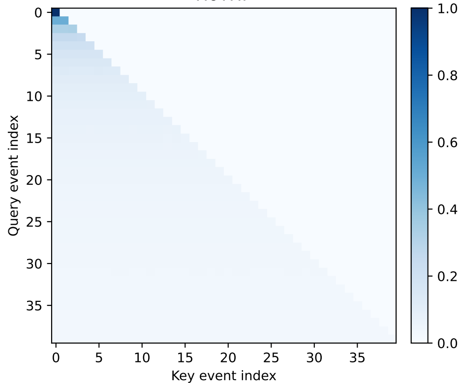
HoTHP
