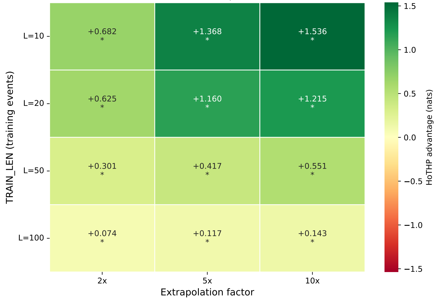
Fast Decay ( \beta=0.5 ) Green = HoTHP better | Wilcoxon test
