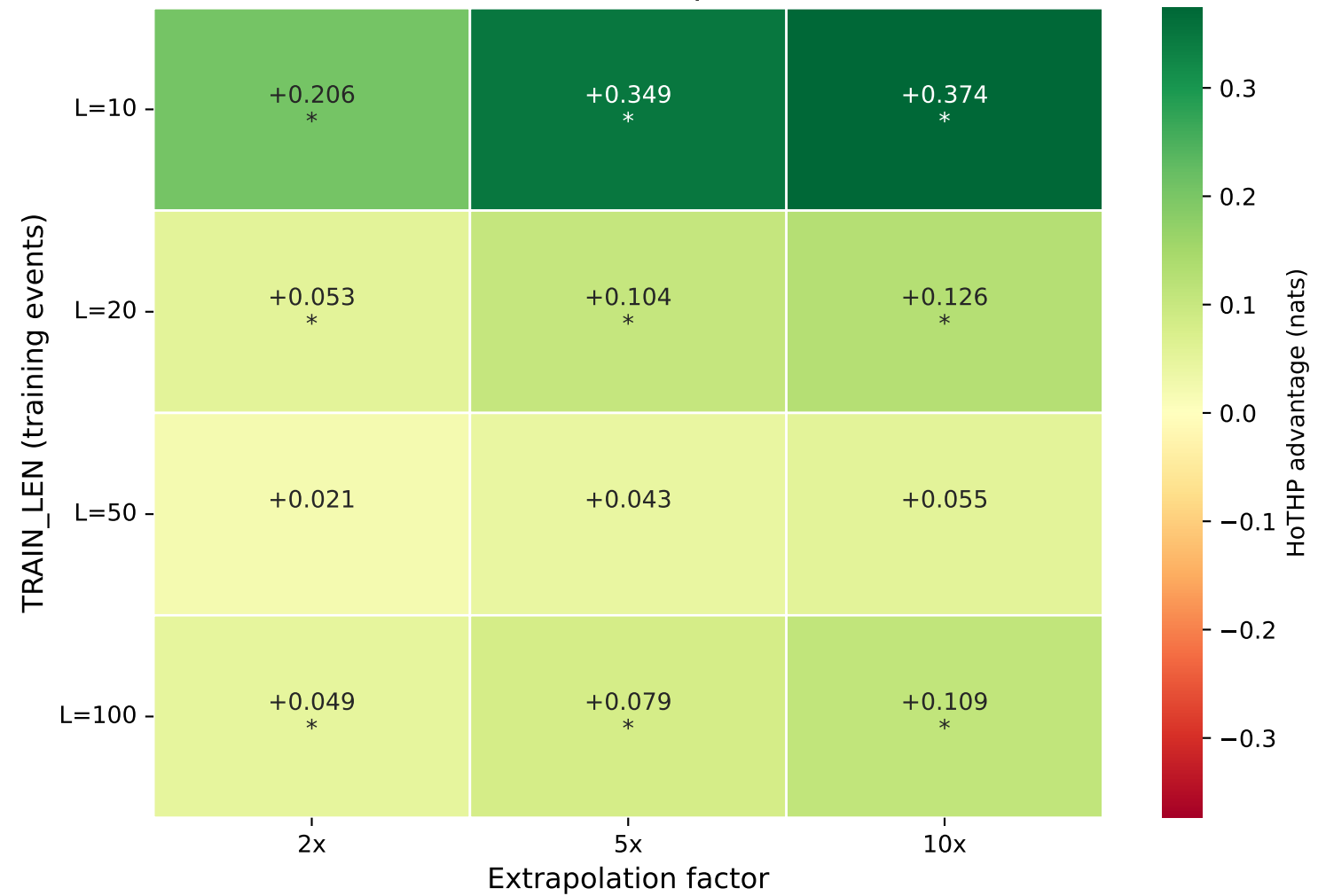
Slow Decay ( \beta=0.02 ) Green = HoTHP better | Wilcoxon test
