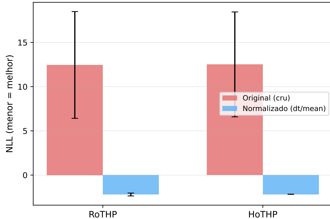
Retweet — 1x (max_len=50)
