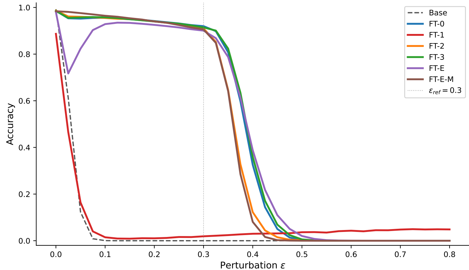
Adversarial accuracy — B30 ablation (PGD L_\infty )
