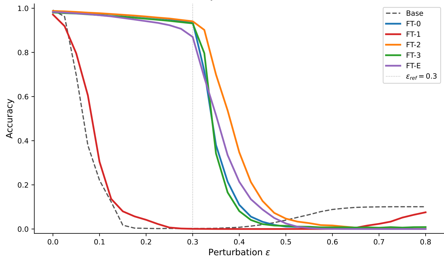
Adversarial accuracy — ProtoVAE ablation (PGD L_\infty )
