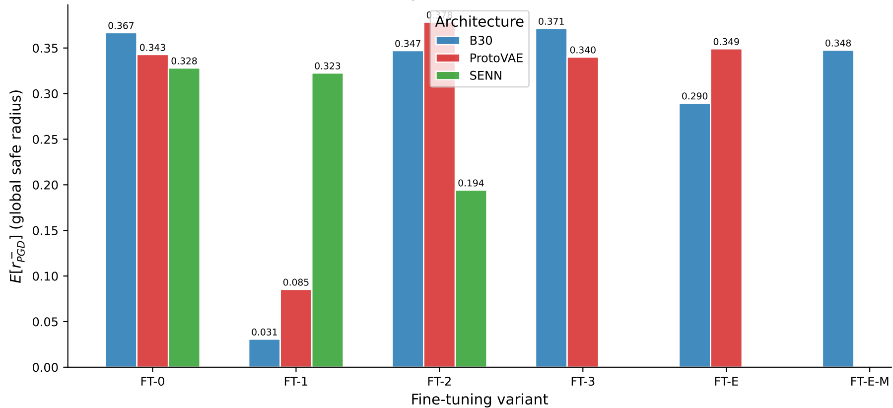
Cross-architecture comparison of E[r_{PGD}^-] (higher = more robust)
