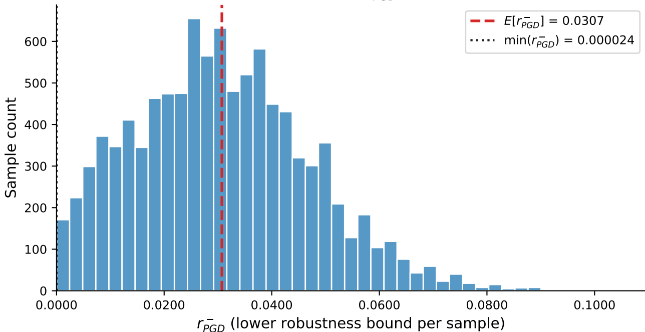
Distribution of r_{PGD}^- — B30
