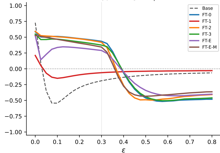
Encoder Drift R_{enc}
