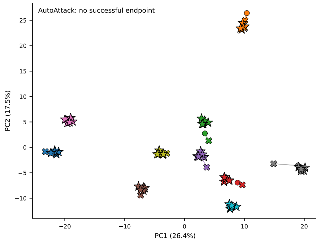
FT-0 ( \epsilon=0.3 , 80 steps)
