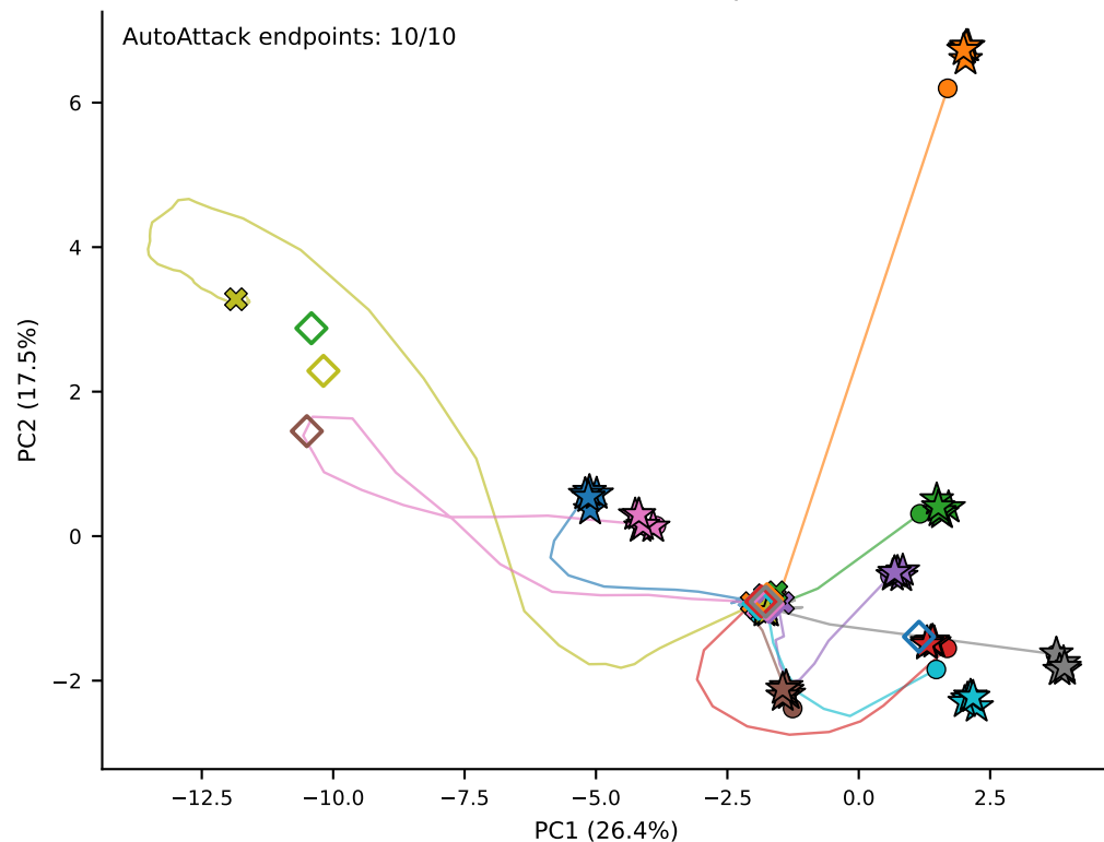
Base ( \epsilon=0.3 , 80 steps)
