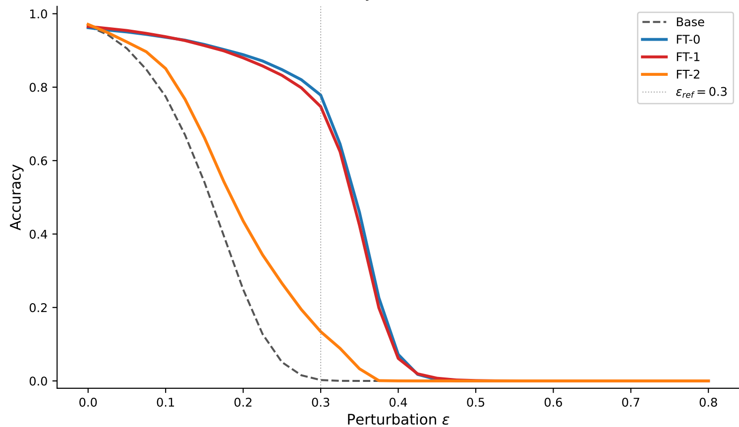
Adversarial accuracy — SENN ablation (PGD L_\infty )
