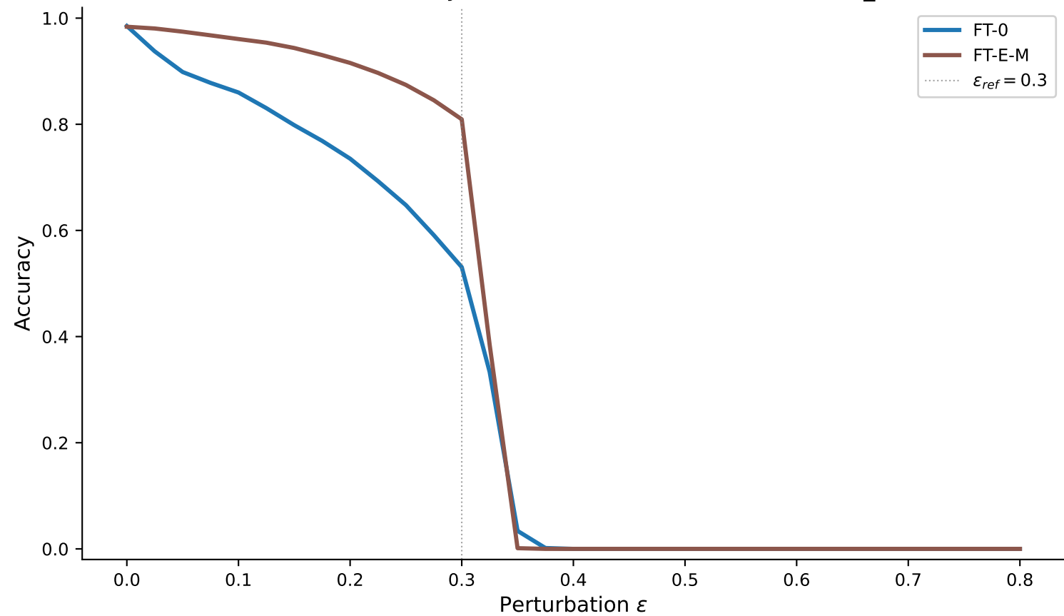
Adversarial accuracy - B30 selected models (AutoAttack_adv)
