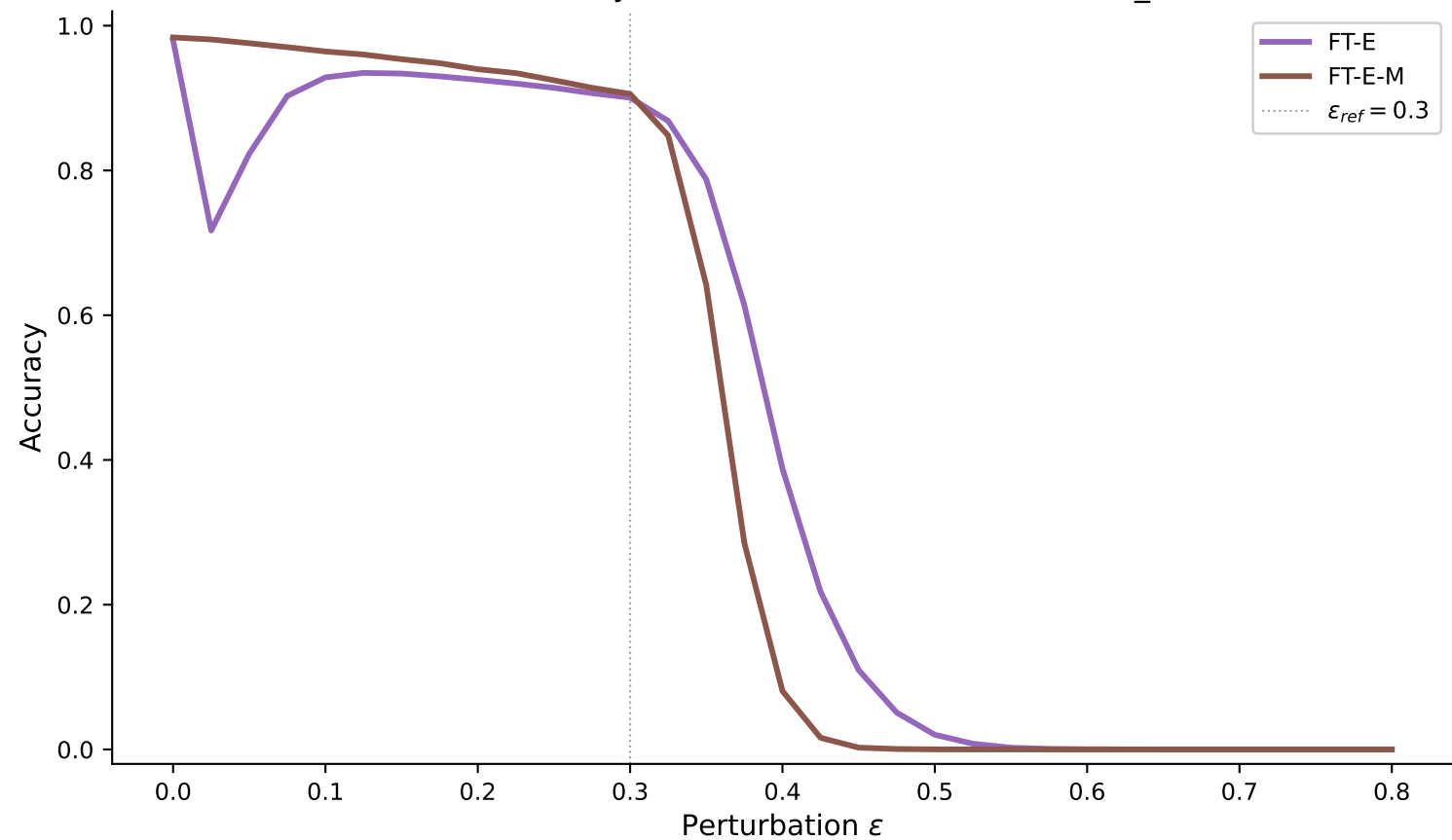
Adversarial accuracy - B30 selected models (PGDInf_attack)
