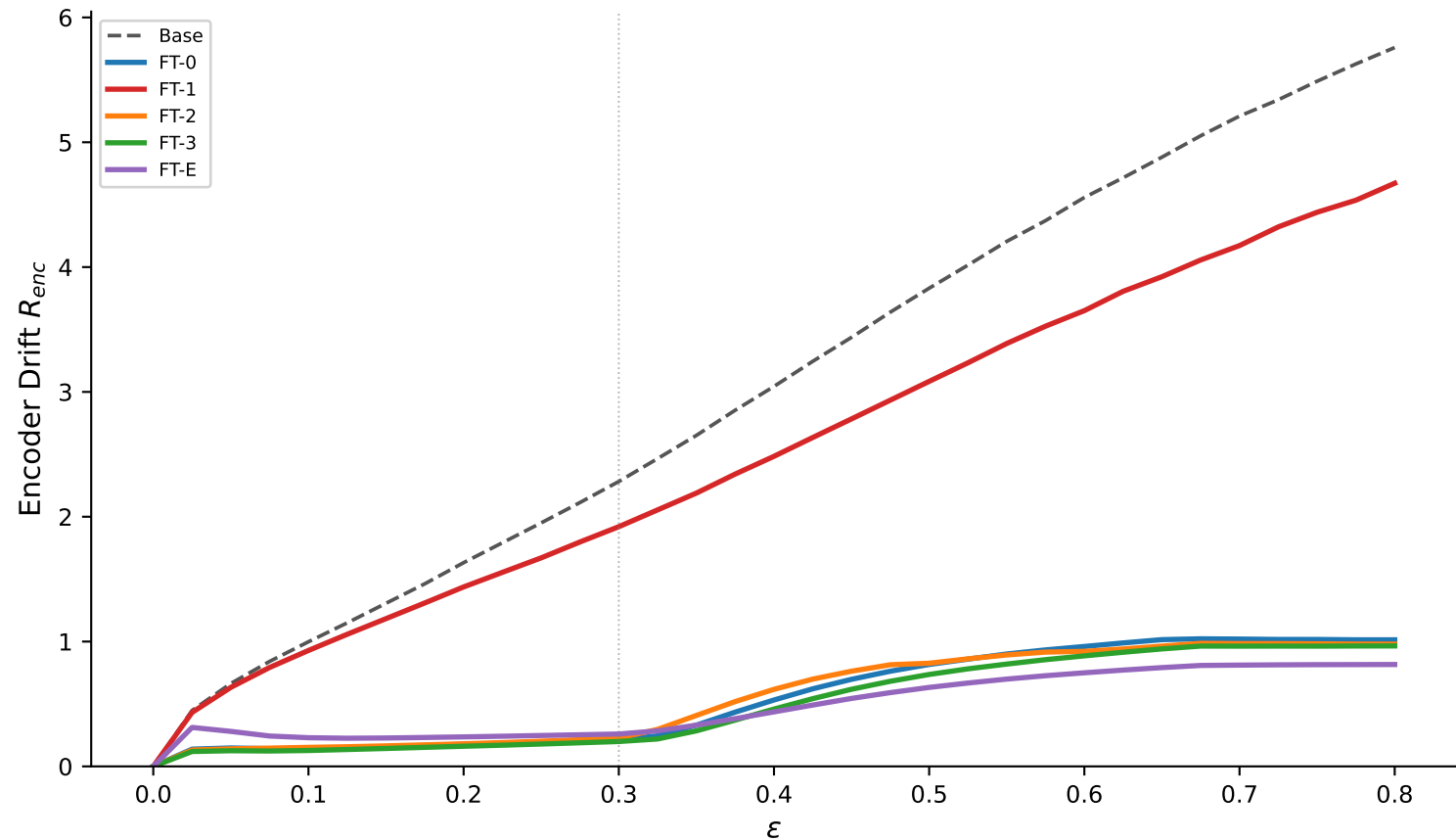
Encoder Drift R_{enc} — B30 ablation
