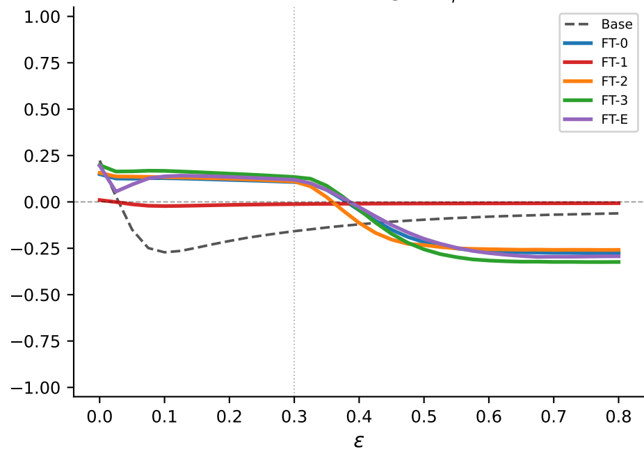
Prediction Margin \tilde{m}_{pred}
