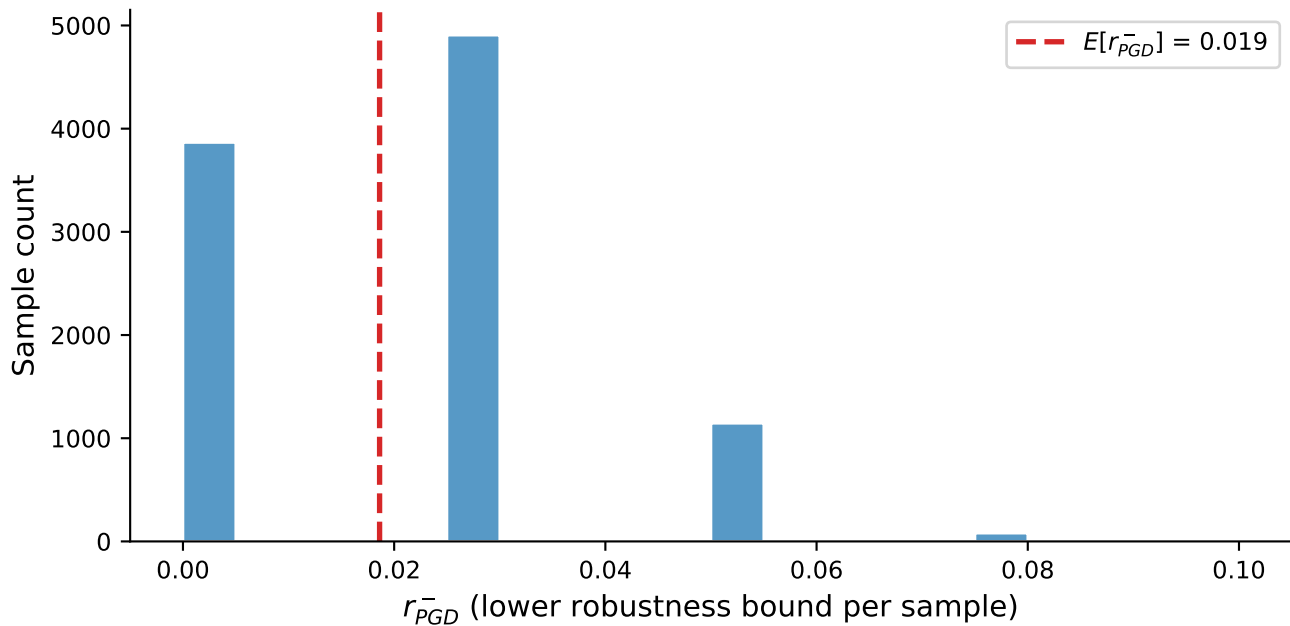
Distribution of r_{PGD}^- — B30 (never-fail fraction = 0.0%)
