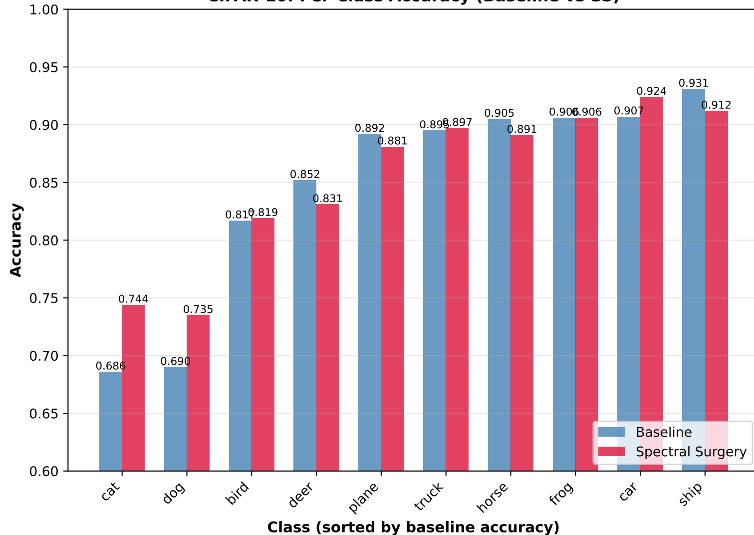
CIFAR-10: Per-Class Accuracy (Baseline vs SS)
