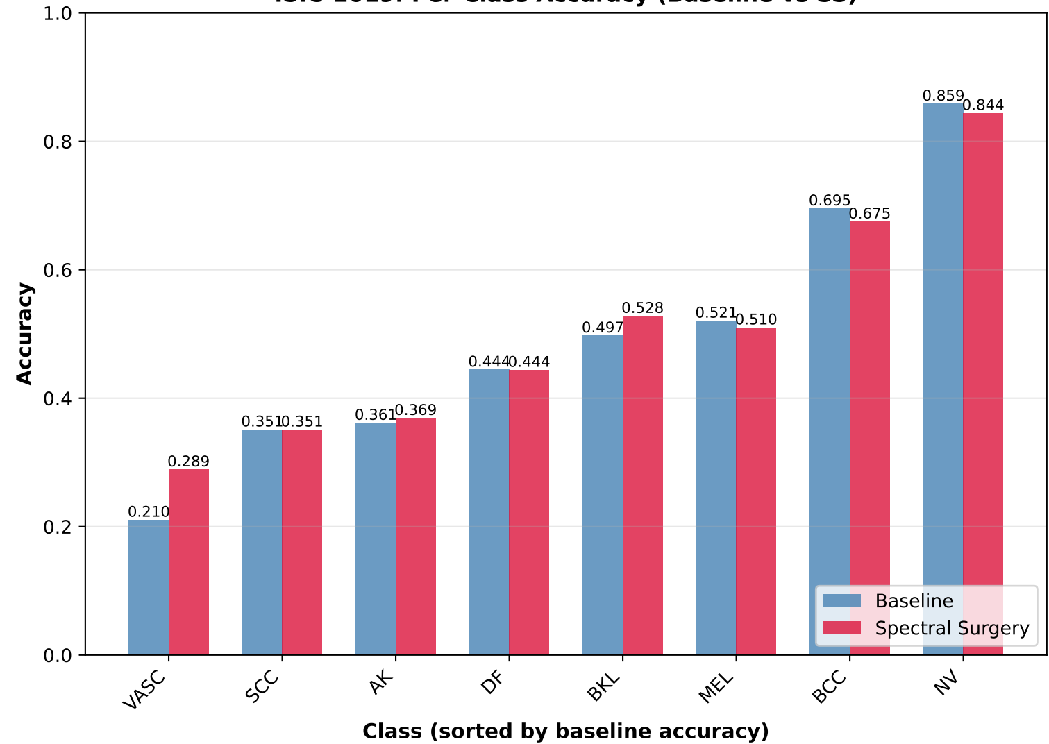
ISIC-2019: Per-Class Accuracy (Baseline vs SS)
