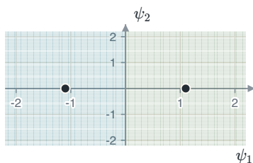
Two points, equal priors: the boundary is halfway.
