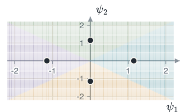
Four points, four boundaries, each perpendicular to the pair it separates.
