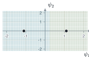
The left symbol four times more likely: its region has grown.
